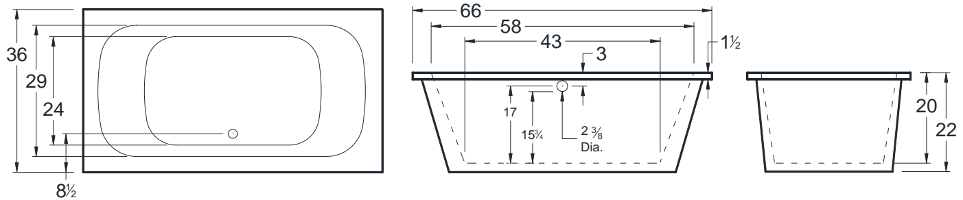
All bathtub dimensions are ± 1/2".
