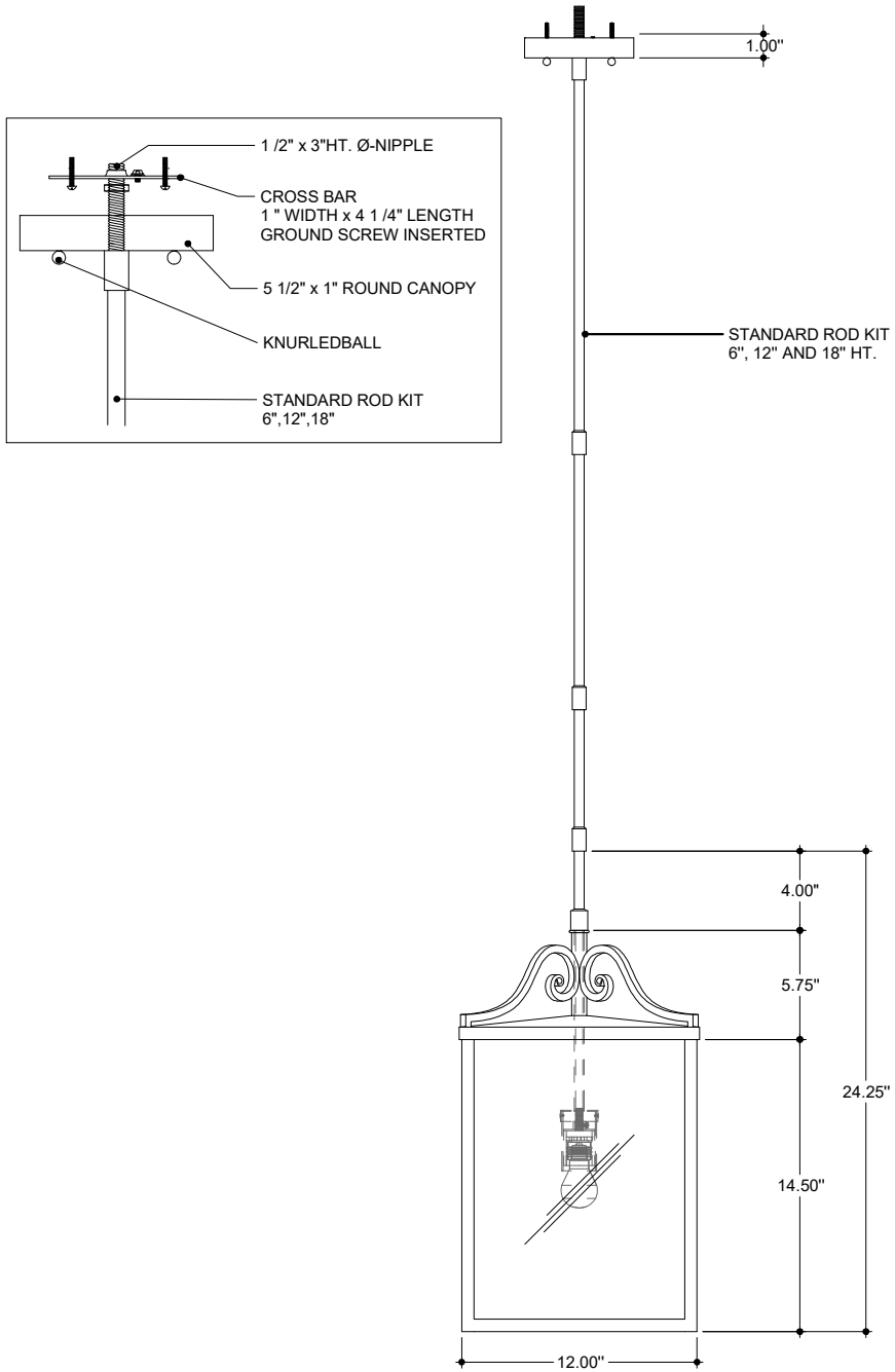
FRONT VIEW
