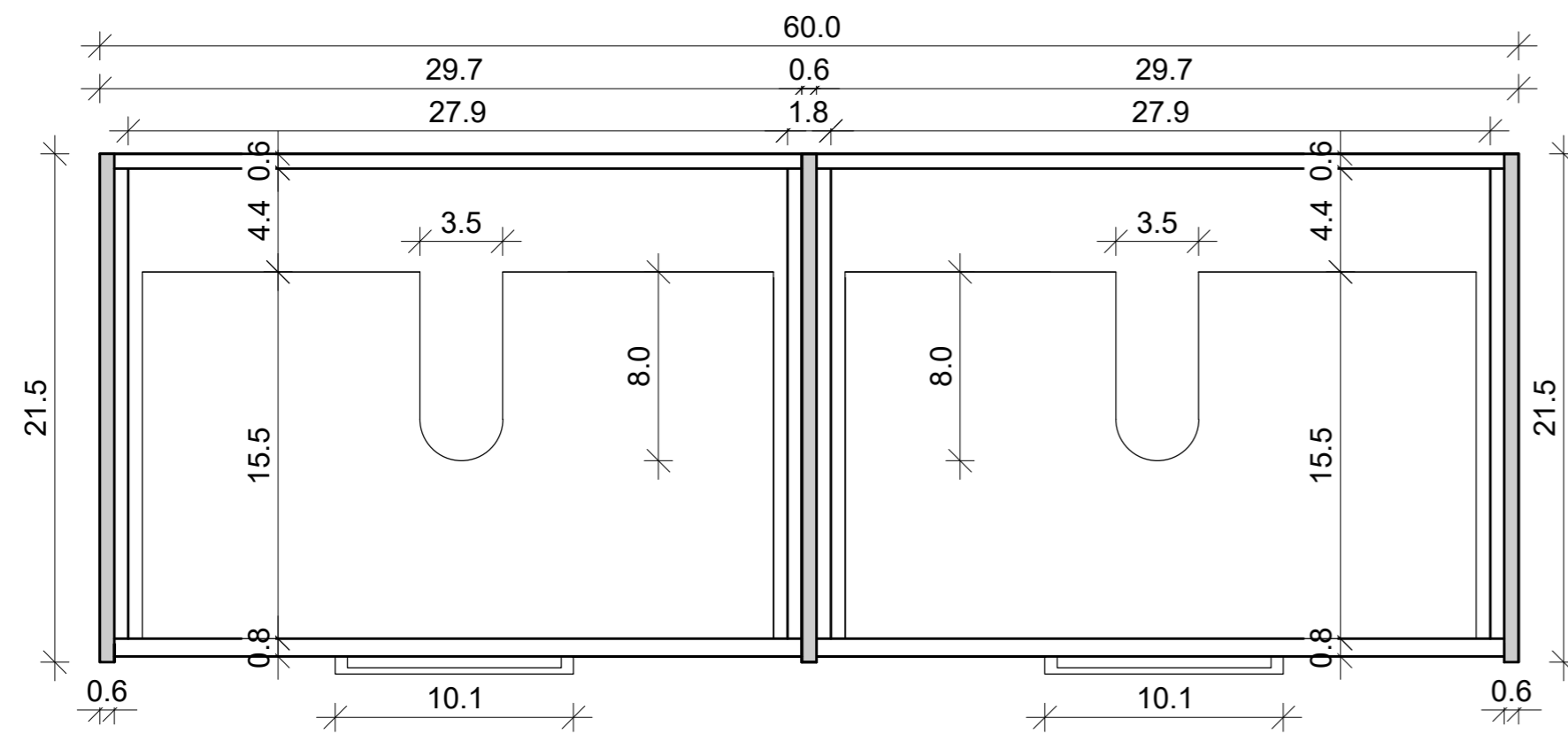
Top View
