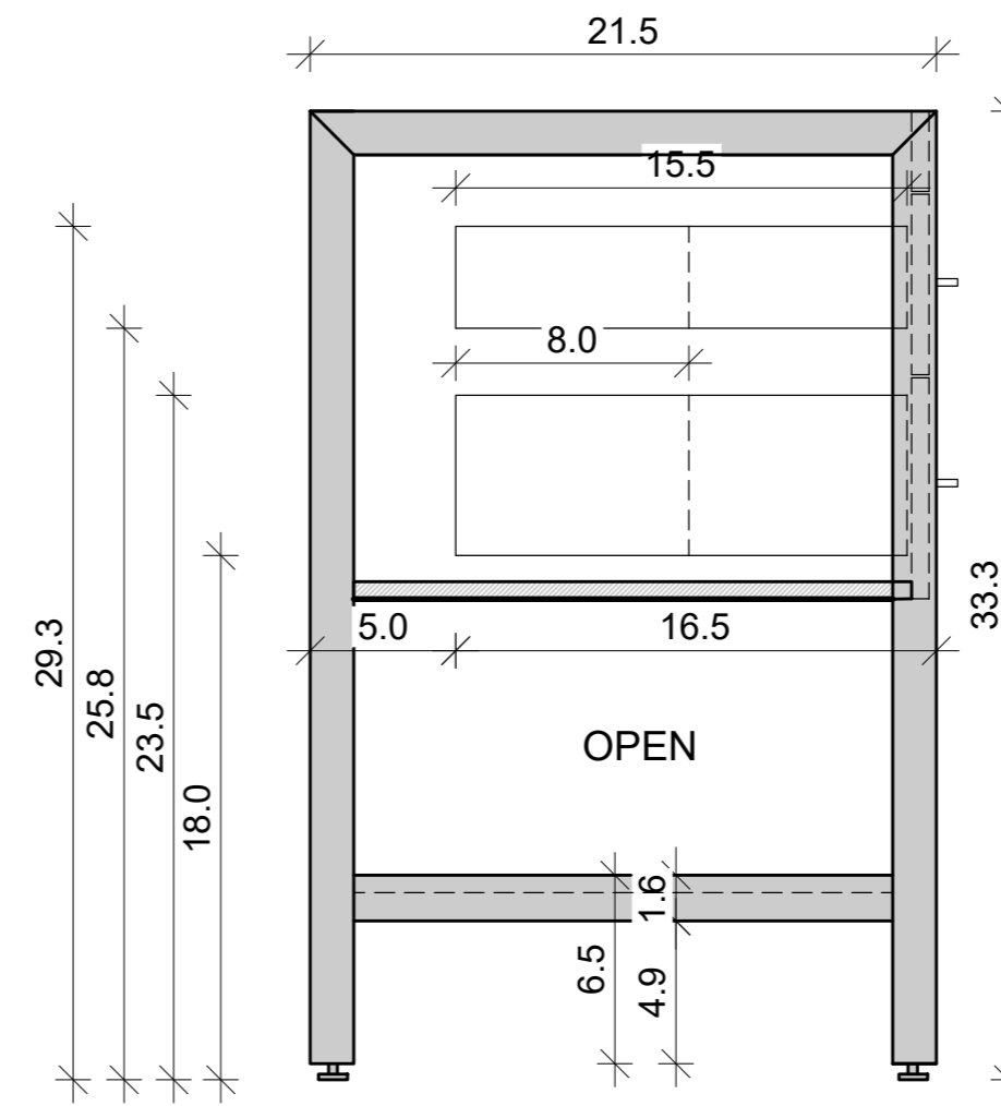
Side View
