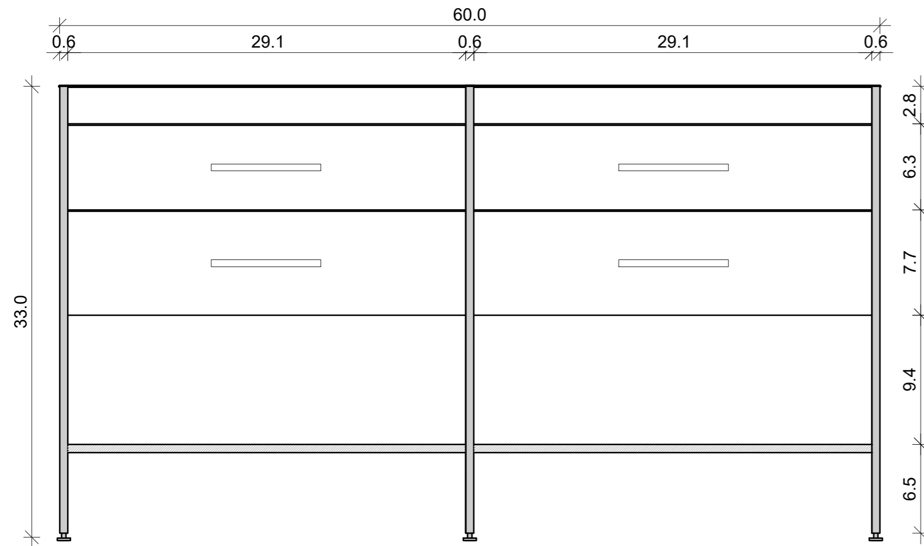
Front View
