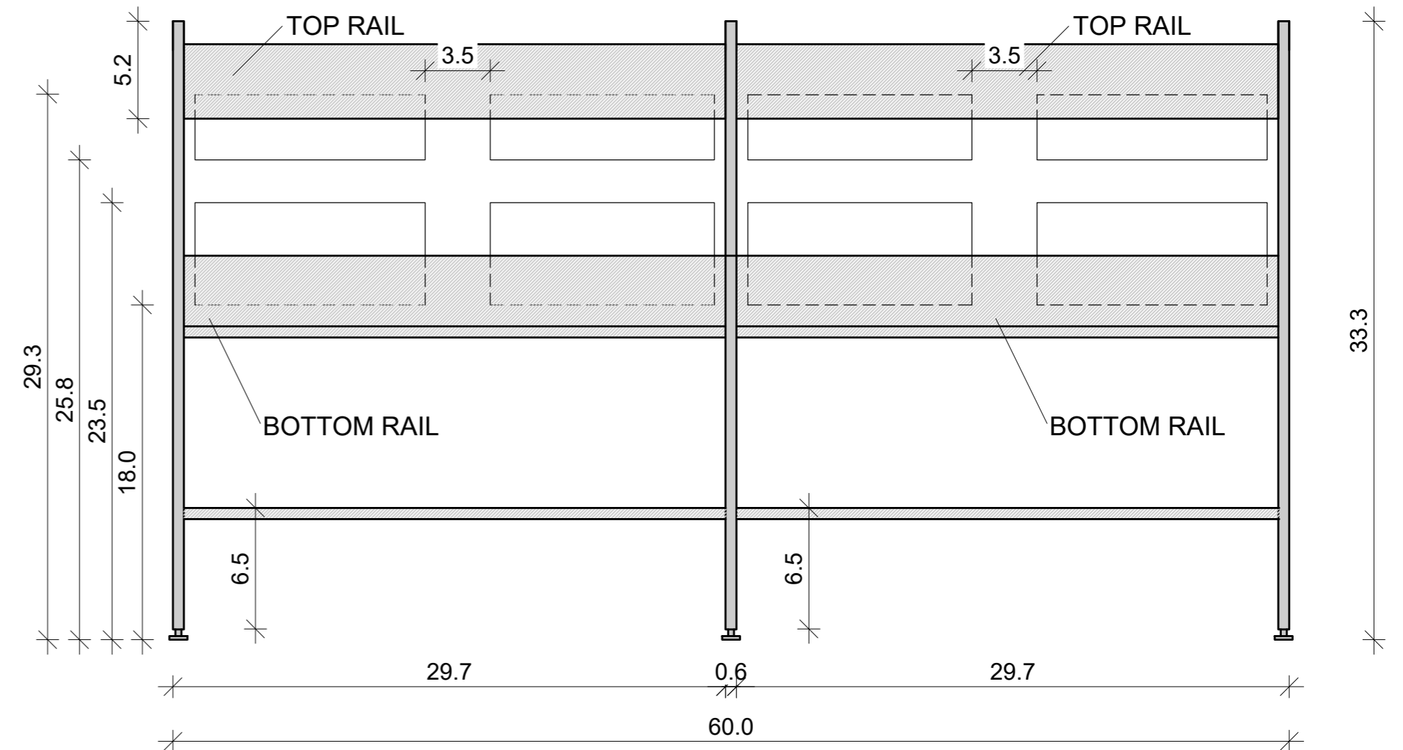
Back View
