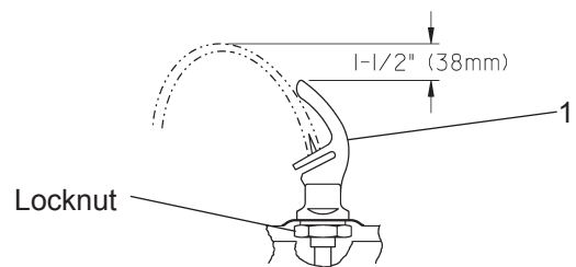
Figure 6 - Bubbler Detail
