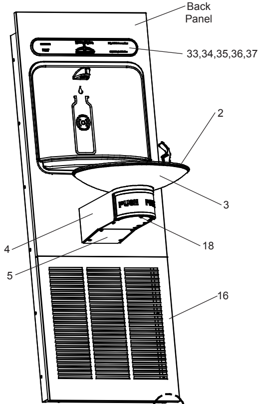
Figure 5 Lower Panel Installation
