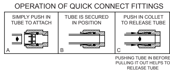
Figure 15 – Quick Connect Fittings
