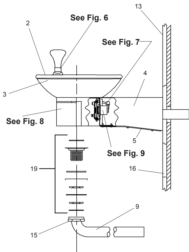
Figure 10 - Drain Assembly
