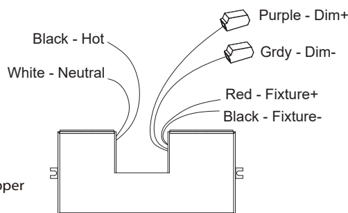
Fig. 3 Driver Wires
